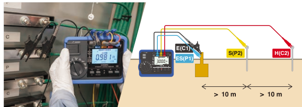
3-pole method using 4-terminal measurement Measure ground resistance values of several ohms or less
