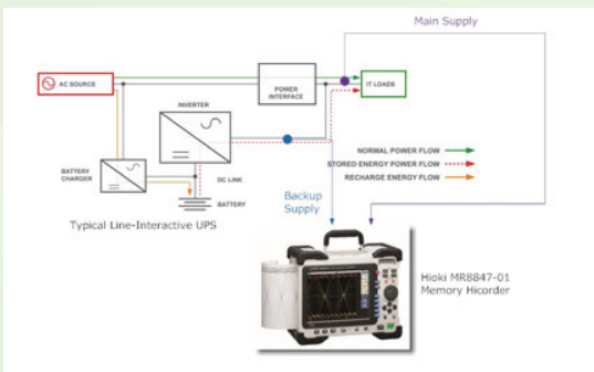
Figure 4: Line-interactive with MR8847-51
