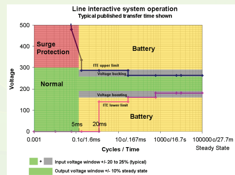
Figure 2: Line-interactive System Ops
