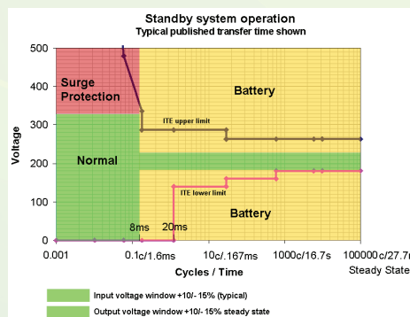
Figure 1: Standby System Ops
