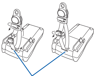
Strap holes
