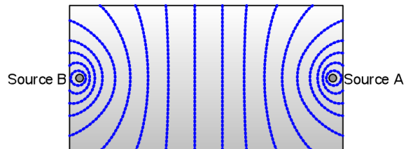
Figure 2. Equipotential Lines on the Measurement Target
