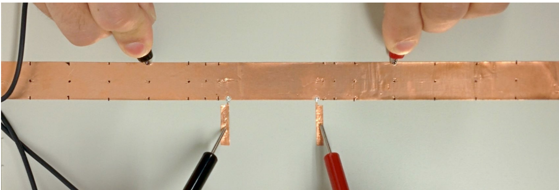
Figure 6. Measurement Positions (Current Application Terminal Positions [Top Edge])
