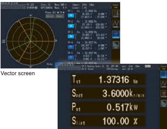
Torque, rpm, motor power, slip
