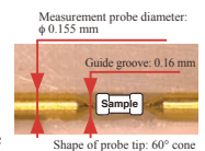
SMD TEST FIXTURE IM9110 Direct connection two-terminal measurement type for measuring SMDs, DC to 1 MHz, measurable sample sizes: 008004 (inch)
