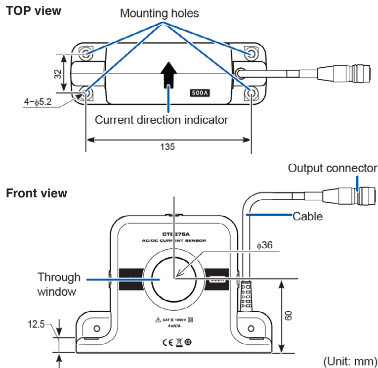
⚡ Figure 5. Dimensions
