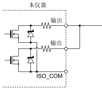
Wired OR
