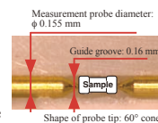
SMD TEST FIXTURE IM9110 Direct connection two-terminal measurement type for measuring SMDs, DC to 1 MHz, measurable sample sizes: 008004 (inch)
