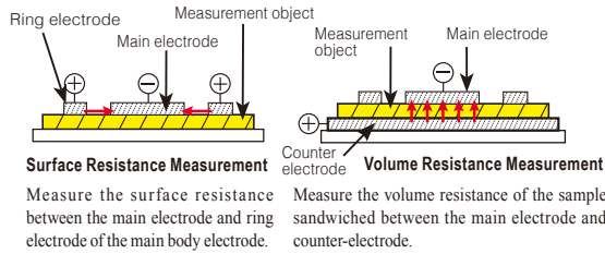
Ring electrode Main electrode
