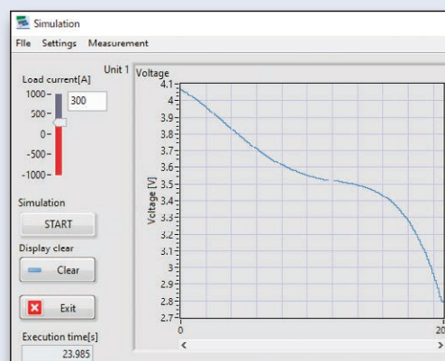
Results of voltage simulation between batteries
