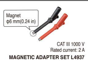
MAGNETIC ADAPTER SET L4937
