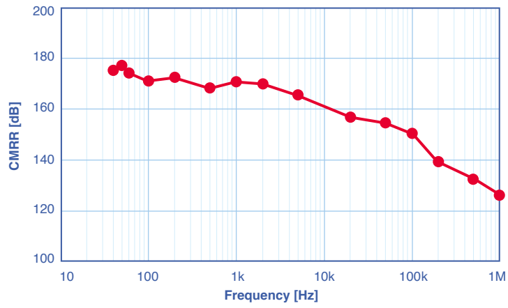
⚡ Figure 4. CMRR characteristics
