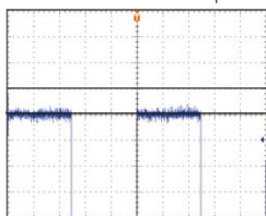
Observed waveform of 15 V output magnified 20x (100 mV/DIV)
