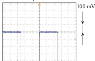
Observed waveform of 15 V output magnified 20x (100 mV/DIV)
