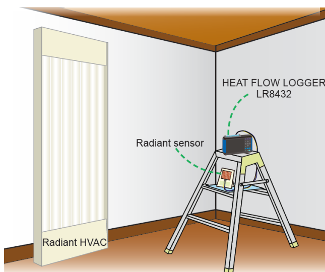
Measurement with the LR8432
