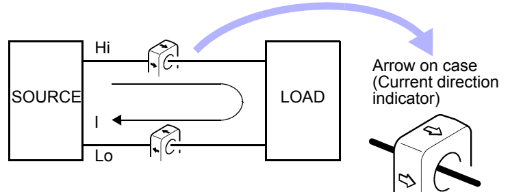
Figure 1. Wiring example
