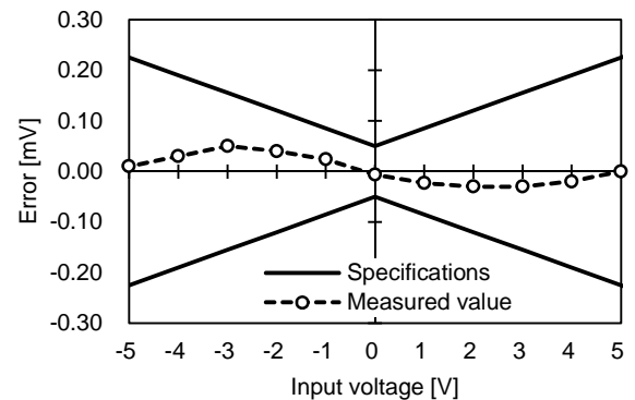
Fig. 13. DC Voltage Measurement Accuracy Linear Characteristics
