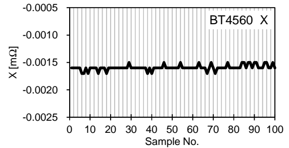
Fig. 5. X Repeatability During 3 m \Omega Resistance Measurement
