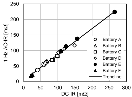
Fig. 16. Correlation Between Low-frequency AC-IR and DC-IR
