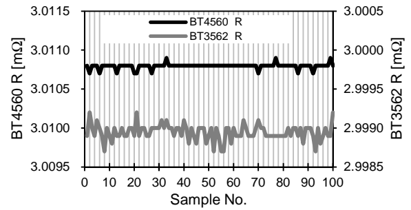
Fig. 4. R Repeatability During 3 m \Omega Resistance Measurement
