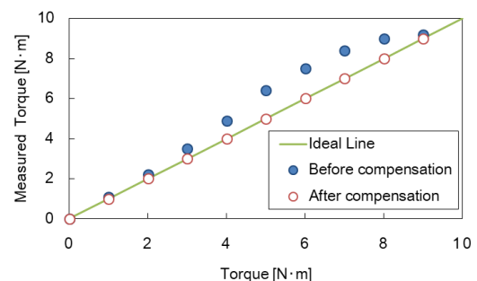
Fig. 12 Compensation of measured torque by the PW8001 (nonlinearity compensation)
