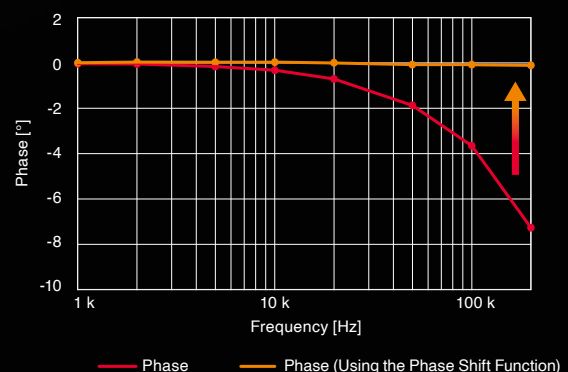
Example of Phase Characteristic Compensation with AC/DC CURRENT SENSOR CT6862-05 (Typical Values)
