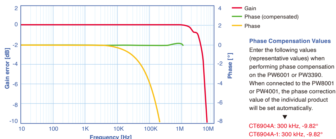
Figure 2. Frequency characteristics
