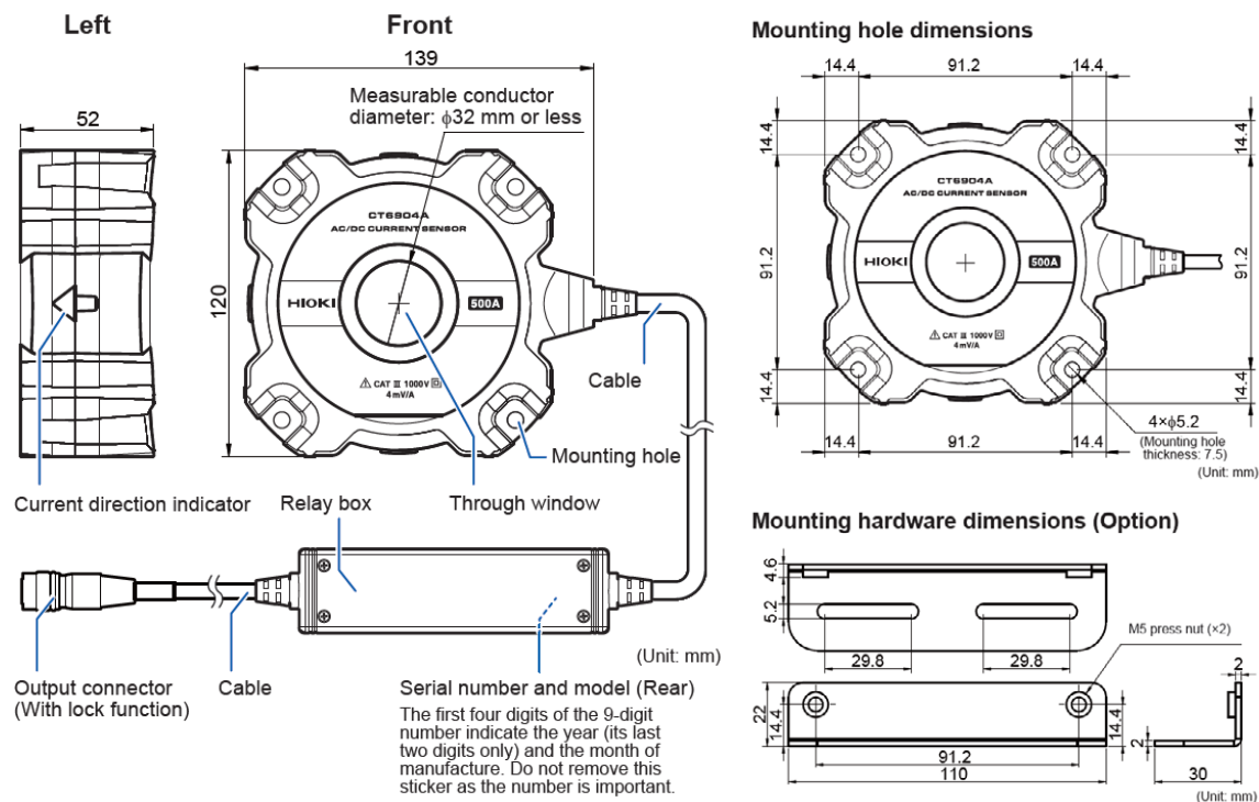
Figure 6. Dimensions
