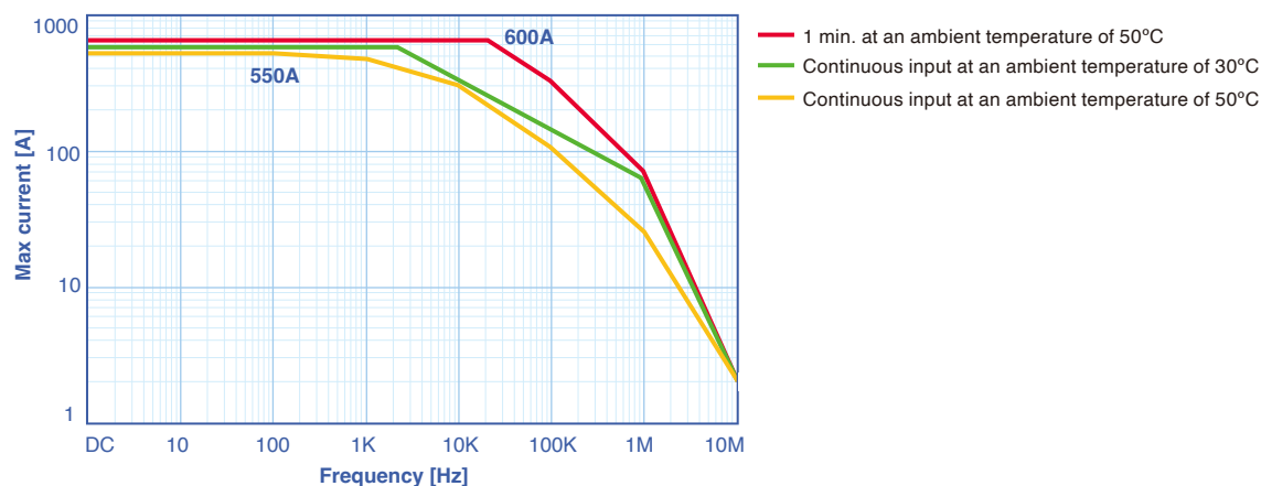
Figure 1. Frequency derating
