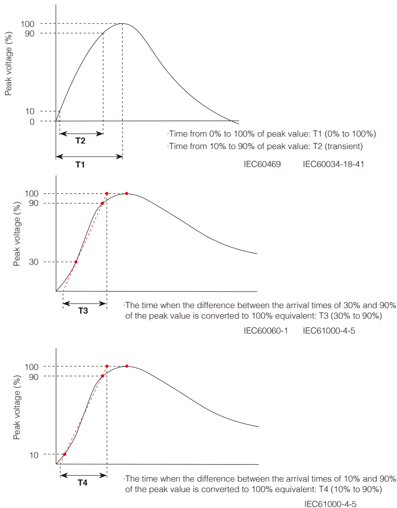
Example rise time displays (with T2 selected)
