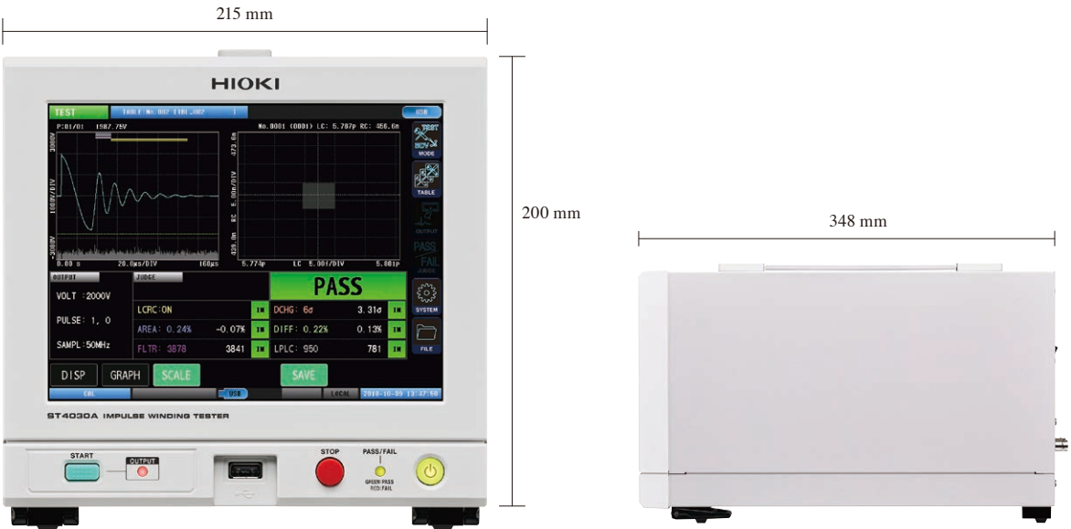
Main unit front
