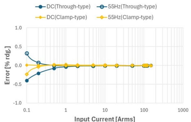
Fig. 7 Linearity
