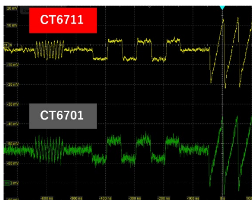
Fig. 11 Output waveform comparison of CT6701 and CT6711
