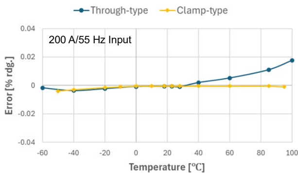
Fig. 10 Gain-temperature characteristics
