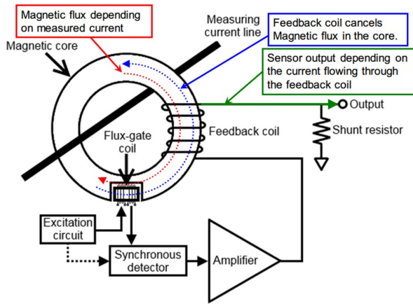
Fig. 3 Zero-flux method (flux-gate type)
