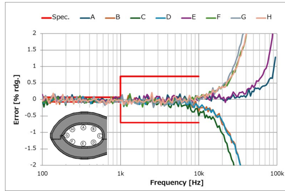
Fig. 5 Gain-frequency characteristics
