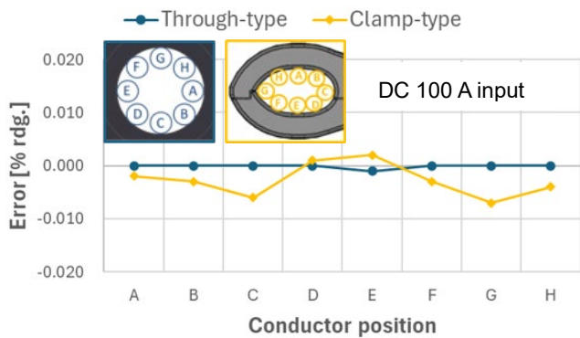
Fig. 8 Effects of conductor position
