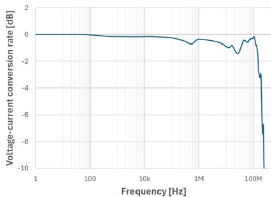
Fig. 12 CT6711 amplitude-frequency characteristics (typical)
