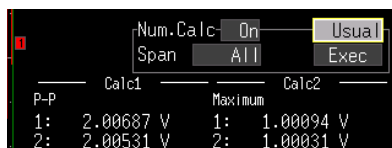
[Usual] display
