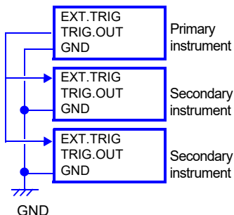
Connection example
