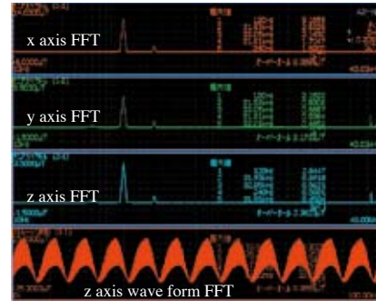
■ 3-channel FFT measurement of IH rice cooker (When the tester is connected to an 8861 Memory HiCORDER.)
